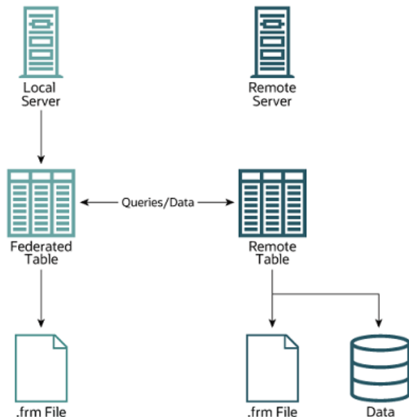
Figure 15.2 FEDERATED Table Structure
