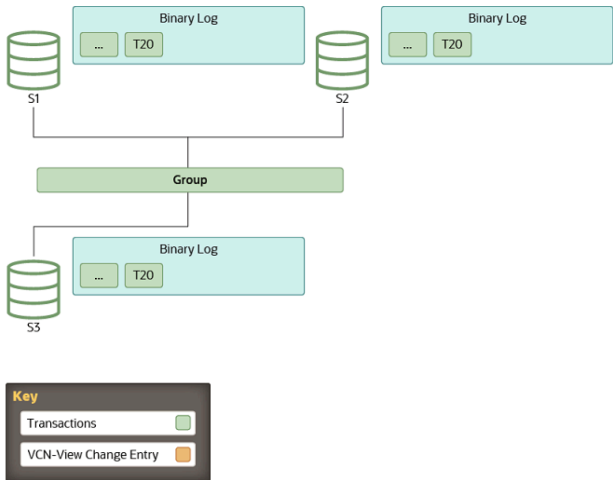
Figure 17.10 Stable Group
